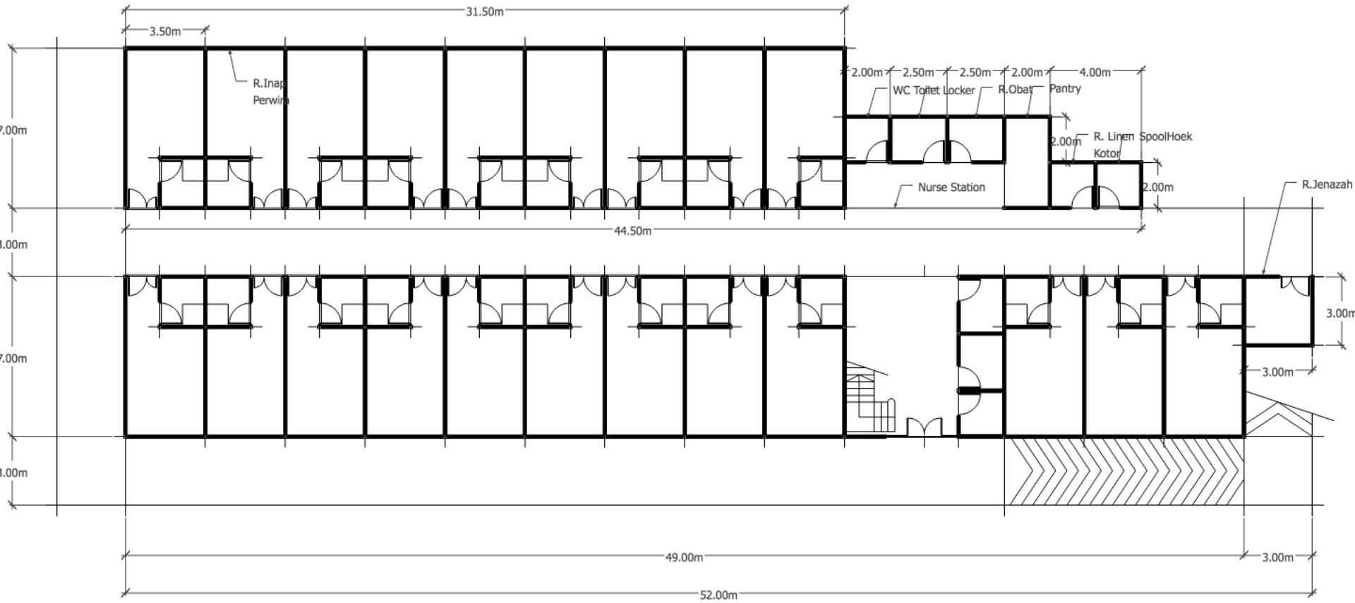
DENAH LT.1 R.INAP PERWIRA RS. DR. SALAMUN-BDG
