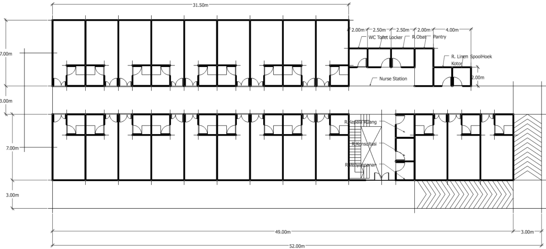
DENAH LT.2 R. INAP PERWIRA RS. DR. SALAMUN-BDG
